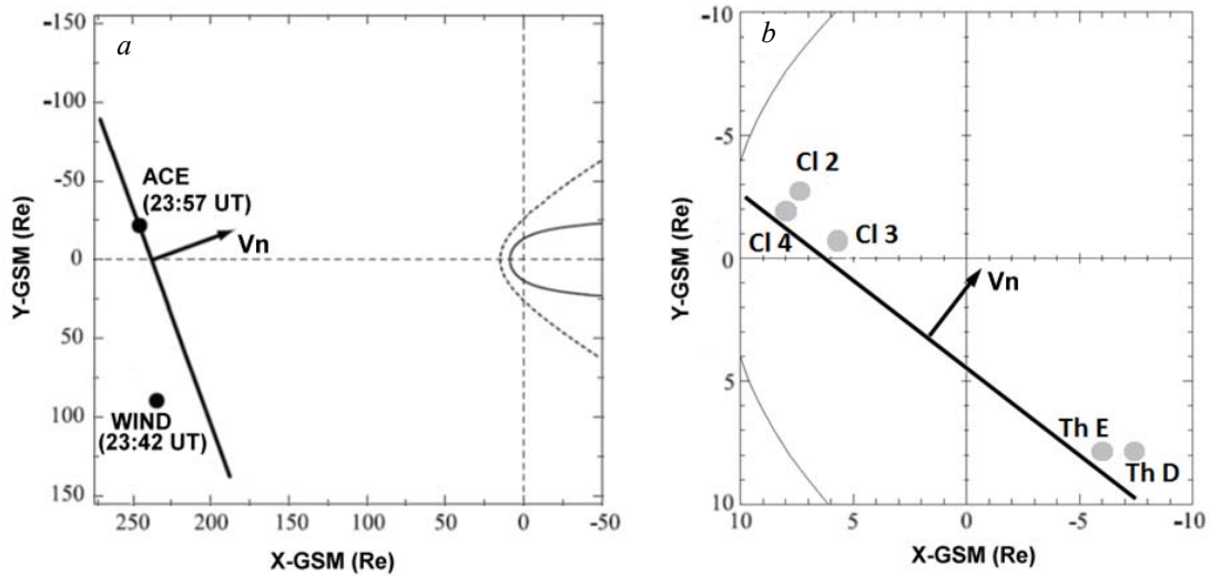
Figure. 2. Satellite location in the GSM XY plane in the interplanetary medium (ACE, WIND) (a) and in the magnetosphere (CLUSTER (CI) 2, 3, 4, THEMIS (Th) D and E) (b). The orientation of the IPS shock front and compression wave front (solid lines)
