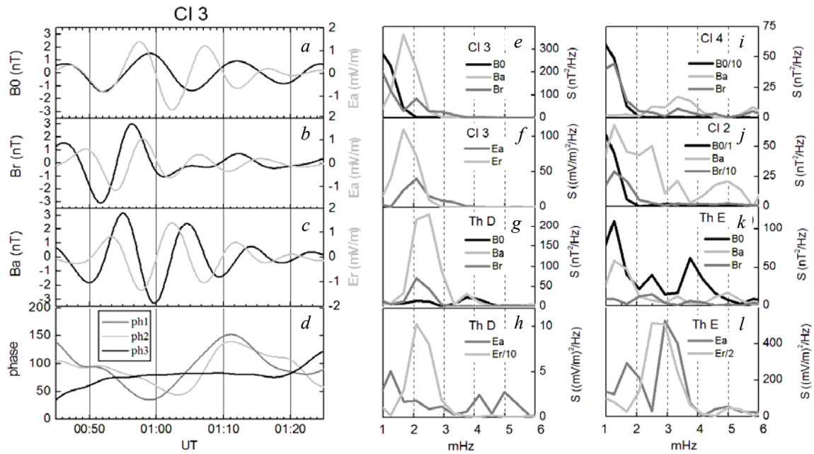
Figure 5. B_0 , B_r , B_a components of the magnetic field (black line) and E_r , E_a components of the electric field (gray line) in the magnetosphere aboard the CI 3 satellite. Magnetic and electric components of compression (a), poloidal (b), toroidal (c) modes and the phase shift between them (d), the frequency spectra of the variations of magnetic and electric fields aboard CI 3 (e, f), Th D (g, h), CI 4 (i), CI 2 (j), and Th E (k, l) at 00:45–01:25 UT.
