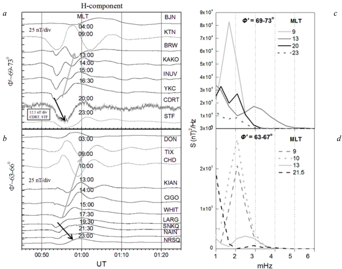
Figure. 3. Variations of the geomagnetic field H component according to data from the stations extended along \Phi' = 69-73^\circ (a) and \Phi' = 63-66^\circ (b) latitudes, frequency spectra of variations (c, d) in the interval 00:45–01:25 UT. Azimuthal propagation to the west (gray arrow) and to the east (black arrow)
