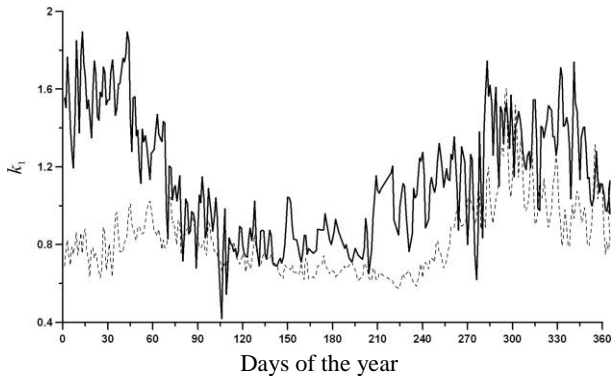
Figure 2. k_1 in 2003 (solid line) and in 2009 (dashed line), 200 km, 12 LT
