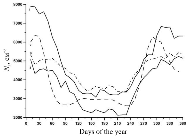
Figure 1. Experimental versus simulated N_e (200 km, 2003, 12 LT): 1 — digisonde; 2 — IRI [Bilitza, 2017]; 3, 4 — SEM [Shchepkin et al., 1997] with different coefficients
