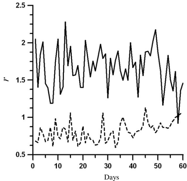
Figure 3. r=N_{ex}/N_{clc} in 2003 (solid line) and 2007 (dashed line), 200 km, 12 LT. Along the X-axis are numbers of winter days in the year
