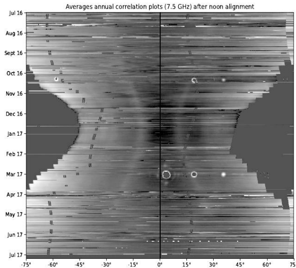
Figure 2. Correlation plots obtained from July 2016 to July 2017. Along the X-axis is the hour angle; the noon is shown by the thin solid line. Dashed black lines indicate SRH diagnostics. The light arcs symmetric about the noon denote correlation plot variations. The circles outlined by white, which are related to observation dates close to the equinox, are responses to the radiation of geostationary satellites
