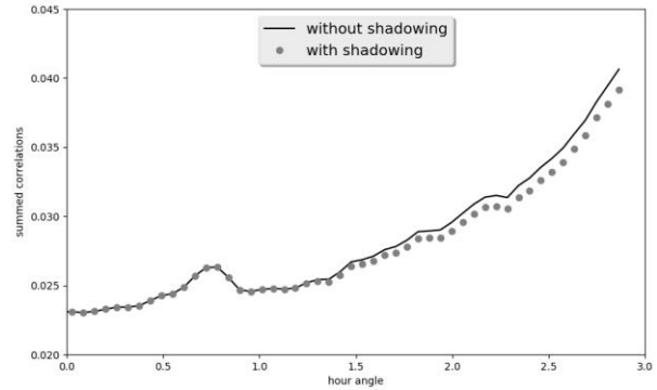
Figure 6. Correlation plot models: without regard for antenna shadowing (solid line); with regard for shadowing ( -23^\circ declination, 7.5 GHz frequency) (circles). Because of symmetry, only half of the correlation plot is shown which corresponds to positive values of the hour angle
