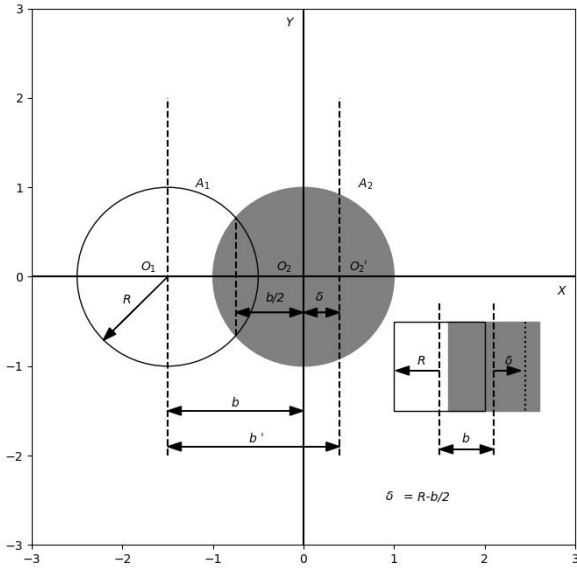
Figure 4. Schematic representation of antenna shadowing. Estimated distance between antennas b is the antenna baseline. If A_1 shadows A_2 , the effective antenna baseline increases: b' = b + \delta , where \delta is the gravity center of the aperture unaffected by shadowing. For the square aperture it is obvious that \delta = R - b/2 , where R is the aperture half size. In the first approximation, this expression can also be used for circular apertures
