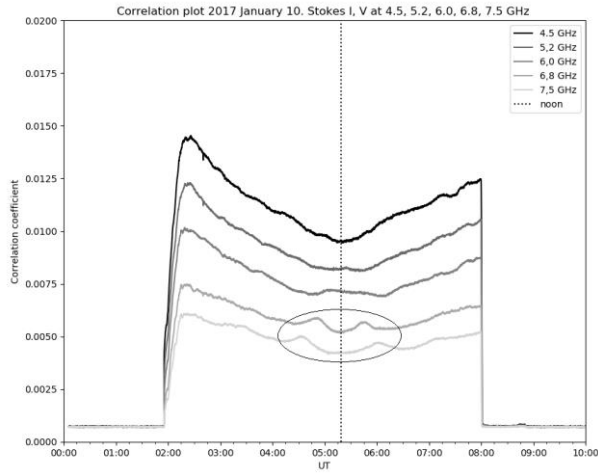
Figure 1. Correlation plot variations caused by changes in the SRH beam pattern. The oval marks variations that can be mistaken for microwave emission flux density oscillations. Diurnal CP variations are clearly visible
