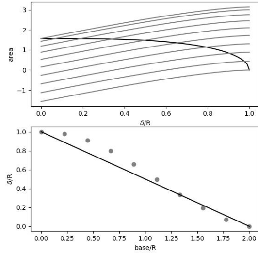
Figure 5. Result of the numerical solution of equation (7). Top panel: the black curve is S_1(\delta) , the gray curves indicate S_2(b, \delta) . Desired \delta values correspond to abscissae of intersections of curves. Bottom panel: circles are the \delta values found, the solid line is the \delta dependence ( b ) obtained in the assumption that apertures are square. It is seen that in the first approximation we can use expression (8) to estimate the antenna baseline change caused by the shadowing
