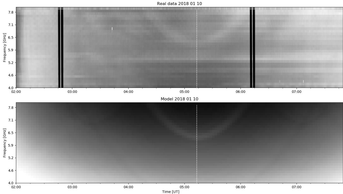
Figure 3. Correlation plots obtained at 32 frequencies in the 4–8 GHz range on January 10, 2018 (top panel): black vertical stripes indicate SRH diagnostics; the white dotted line is the noon; the correlation plot variations are particularly pronounced in the time interval 04–06 hrs at high frequencies. Model correlation plots (bottom panel) calculated in the SRH full frequency band 4–8 GHz for January 10, 2018
