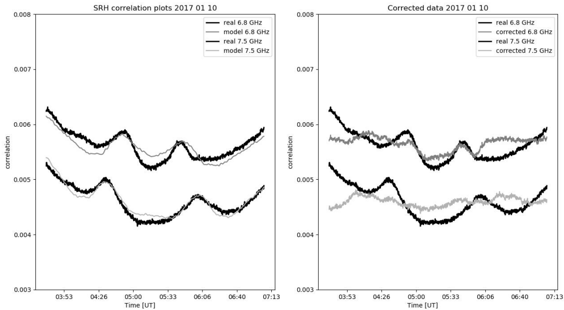
Figure 8. Result of the correction of correlation plots through model ones, calculated as a response to the solar disk (6.8 and 7.5 GHz): original plots (black curves); correction result (gray curves). The CP variations can be reduced several times to the flux density level of \sim 0.1 s.f.u.
