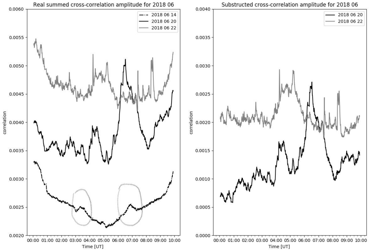
Figure 7. Correlation plots for June 14, 20, 22, 2018 (left); there was no activity on June 14; the active region NOAA12715 appeared on the disk on June 20 and 22. Ovals mark correlation plot variations caused by the response to the solar disk. The result of subtracting the correlation plot for June 8 from the plots for June 20 and 22 (right)
