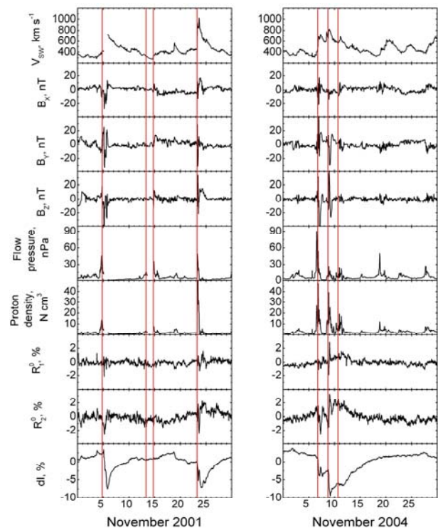
Figure 1. Parameters of IMF B_x, B_y, B_z , solar wind speed V_{sw} , flow pressure and proton density, first R_1^0 and second R_2^0 spherical harmonics and isotropic intensity dl in November 2001 and November 2004
